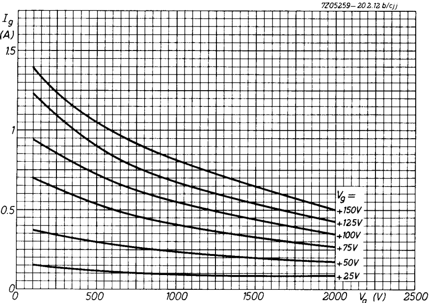
Fig. 3 I_g/V_a characteristics.
