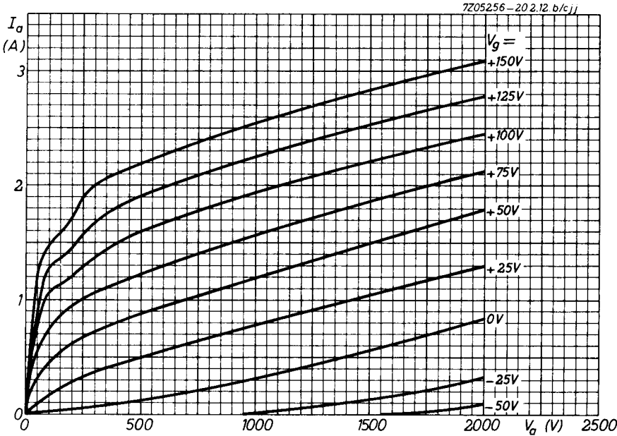
Fig. 2 I_a/V_a characteristics.
